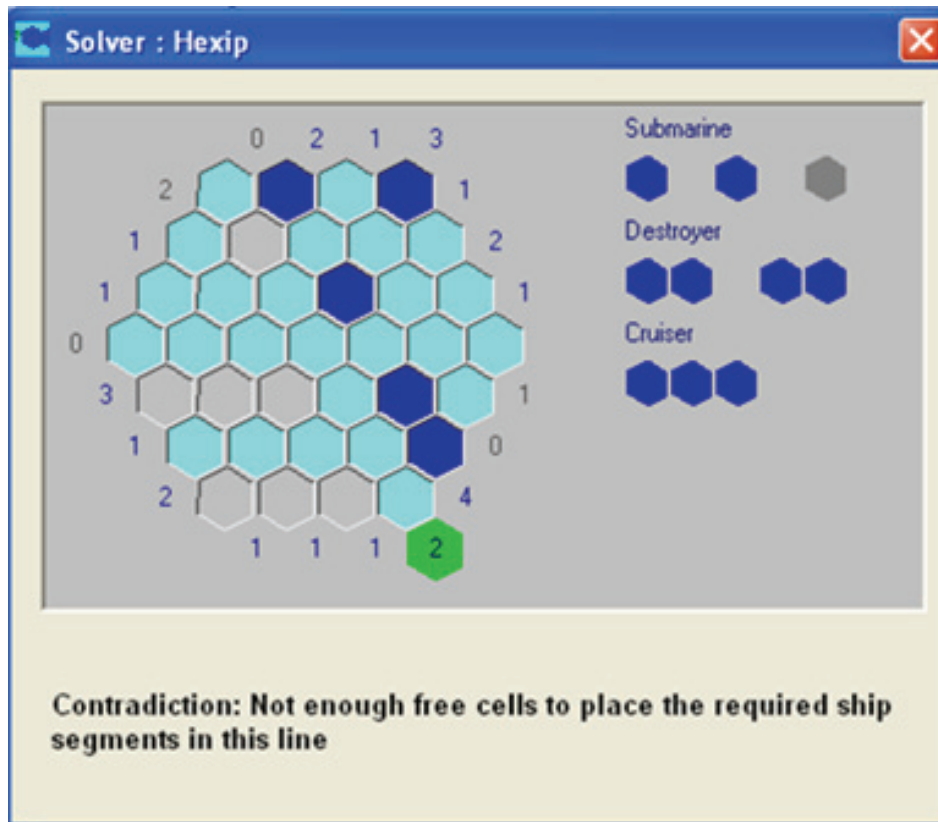
Figure 2: Screenshot showing contextualized feedback
