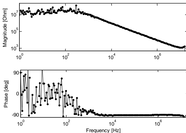
Fig. 4. Impedance spectroscopy of the insulation sample.
