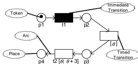
Figure 15: Example of a Timed Petri Net
