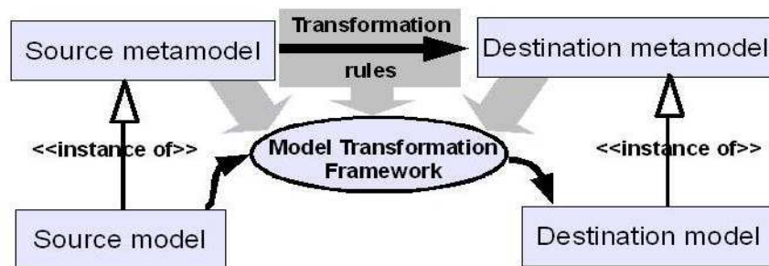
Figure 4: Model Driven Development
