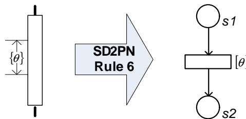
Figure 16: Rule 6 of SD2PN
