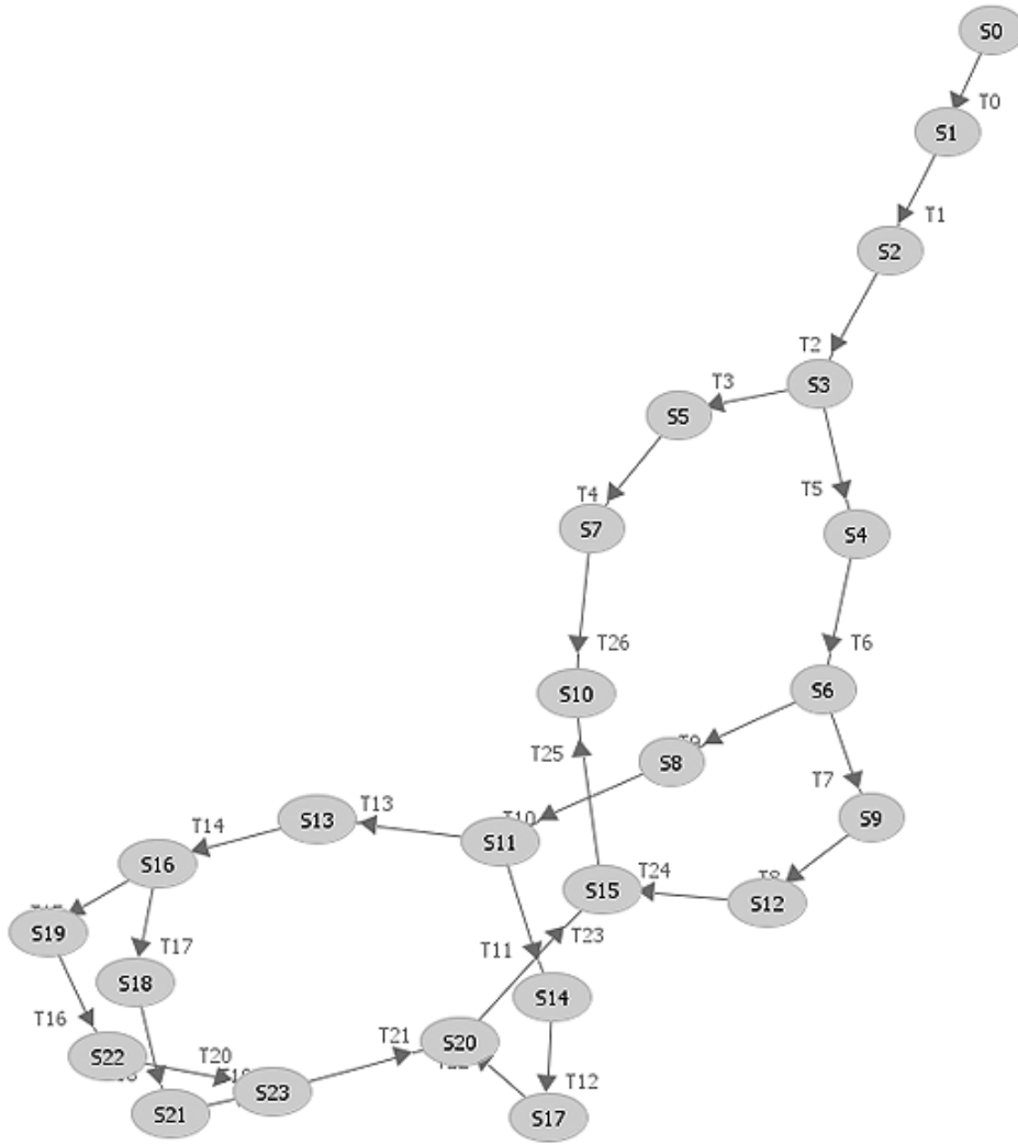
Figure 11: Reachability Graph generated using PIPE
