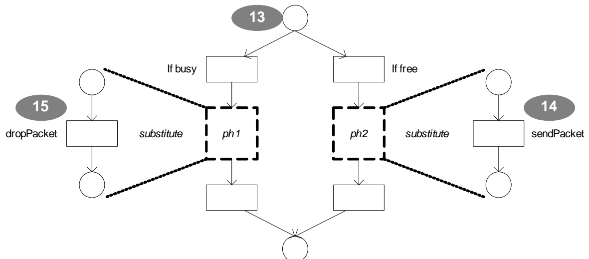
Figure 9: Example of substitute in SD2PN
