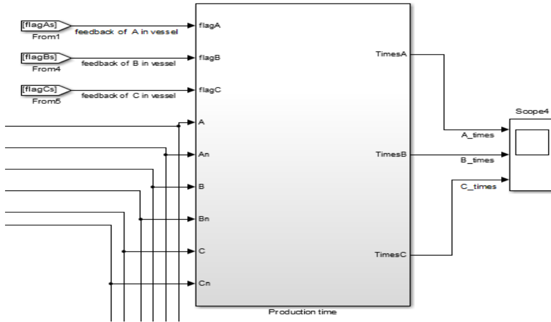
Figure 5.20: Subsystem of production time
