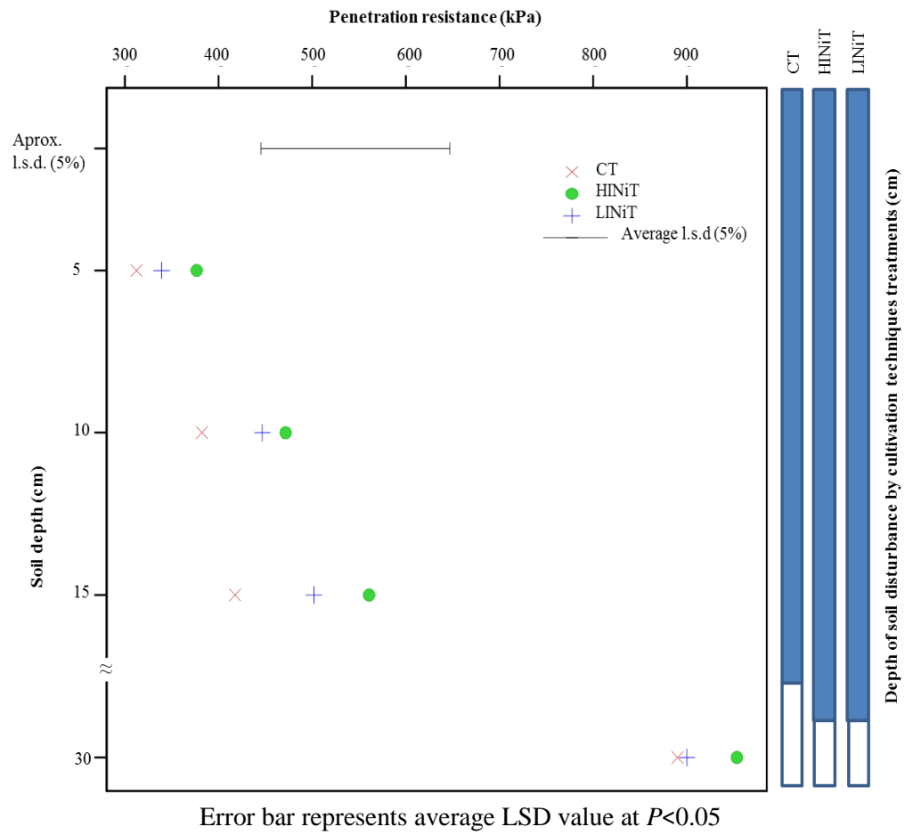
Figure 5. 34. Effect of cultivation techniques and soil depth interaction on soil penetration resistance (kPa) (March 2014) with cultivation techniques soil disturbance depth
