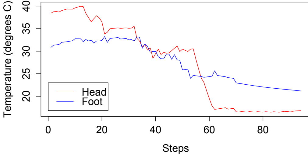
Figure 6.17: Cooling down scenario using Sarsa( \lambda ).
