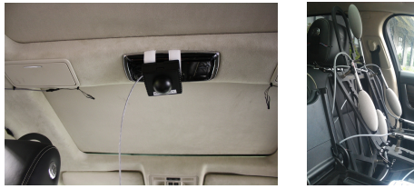
Figure 1: Experimental data gathering. Left: Mean radiant temperature sensor. Right: Upper body of the Flatman thermal manikin.
