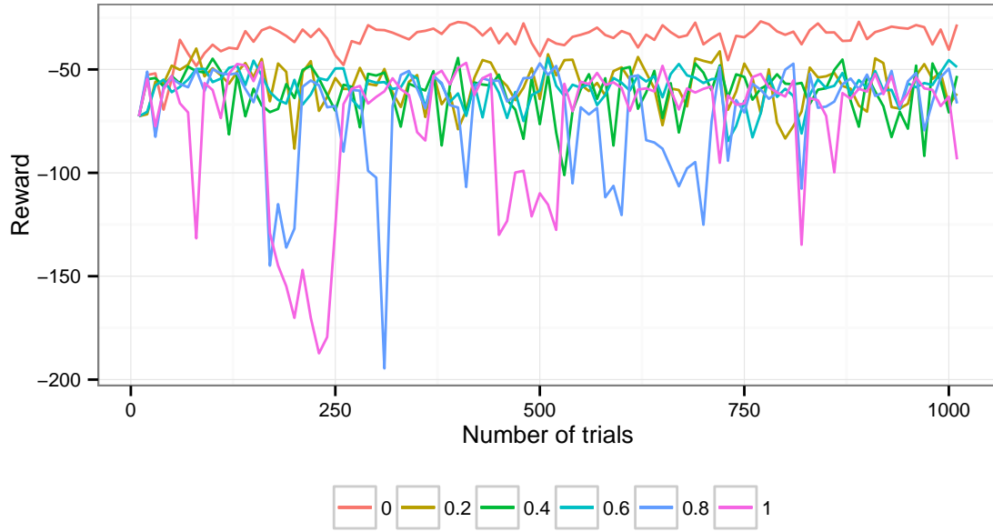
Figure 6.12: Sensitivity analysis on the \varepsilon parameter (values of 0, 0.2, 0.4, 0.6, 0.8 and 1, respectively) on the controller's performance over 1,000 trials.
