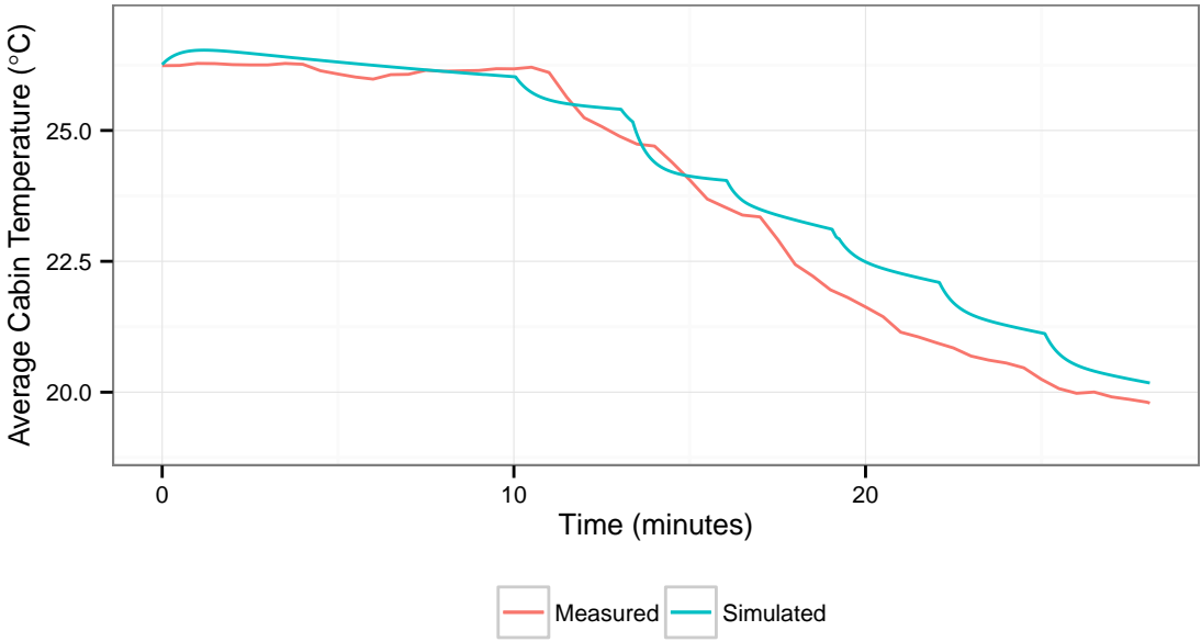
Figure 6.2: Simulated versus measured average cabin temperature during a cool-down scenario.
