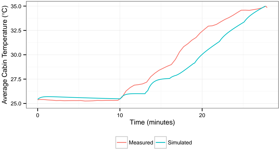
Figure 6.3: Simulated versus measured average cabin temperature within a warm-up scenario.
