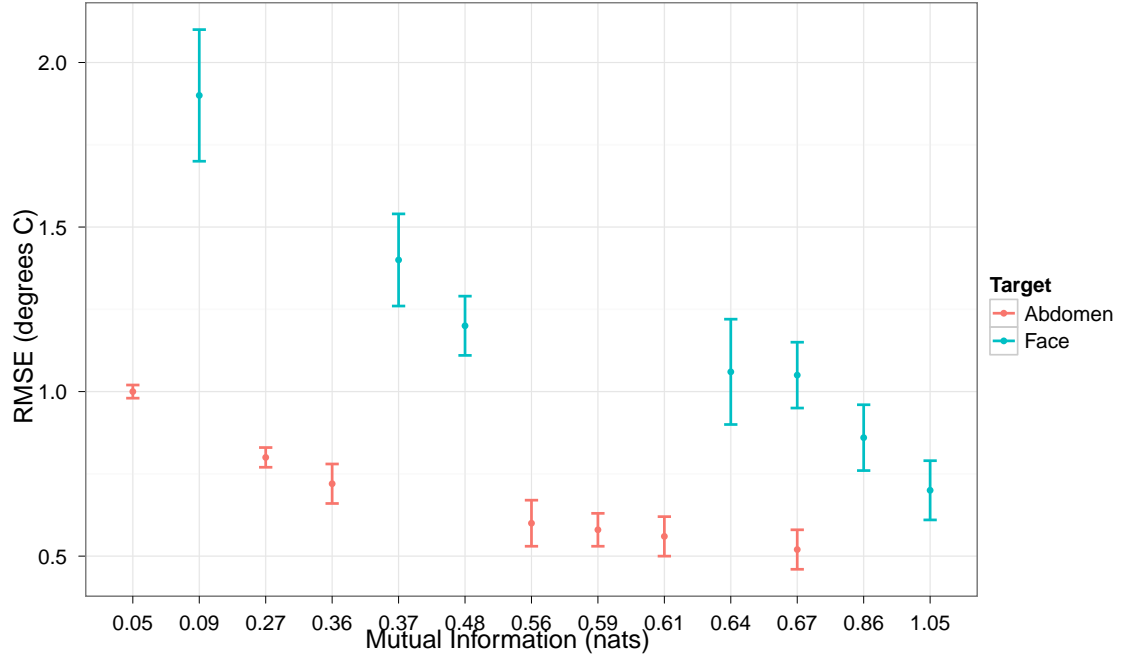
Fig. 3. MI values and their corresponding estimation accuracy
