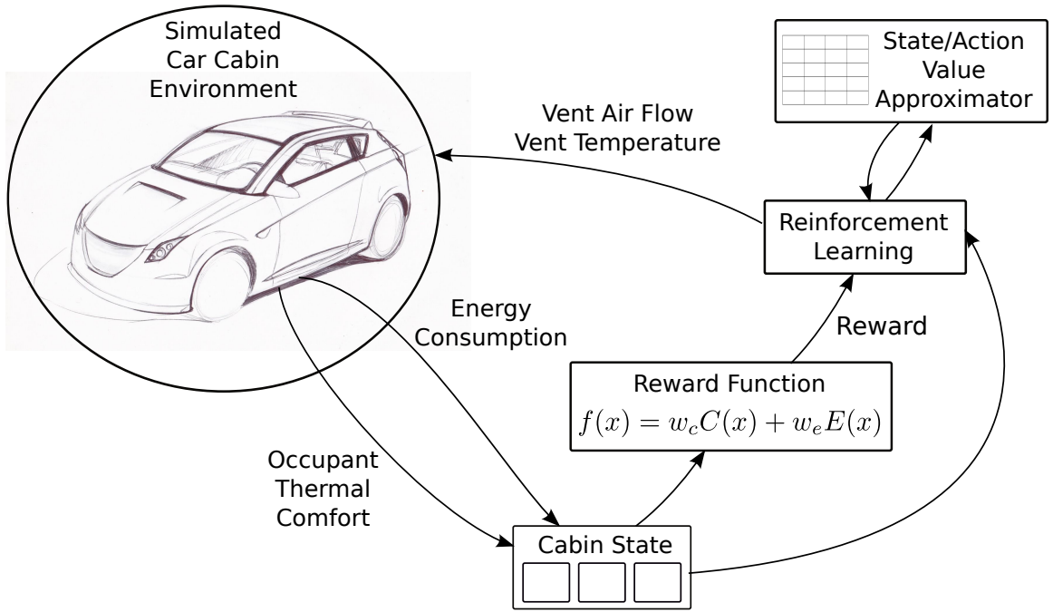
Figure 3.1: Overall simulation-based system architecture.
