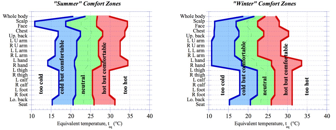
Figure 2.1: Nilsson's clothing-independent thermal sensation diagrams [115].
