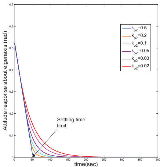
Fig. 10: Attitude response of the gain-scheduled min-norm controller by varying the gains of the high gain mode.
