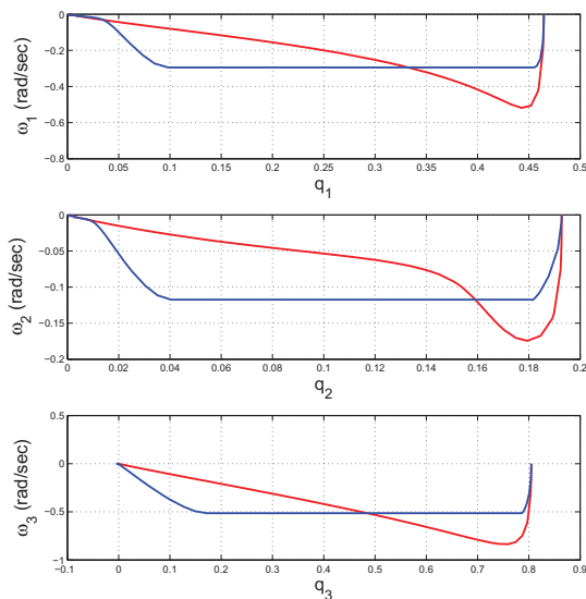
Fig. 6: Phase space trajectory with the gain scheduled and the Krstic/Tsiotras controllers.
