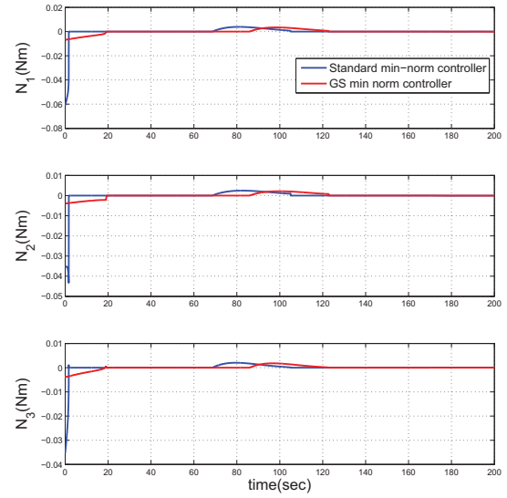
Fig. 3: Control torque of the minimum norm controller, with and without gain scheduling.
