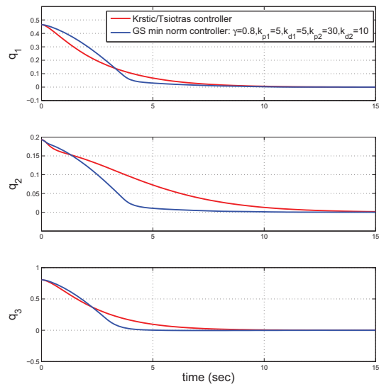
Fig. 5: Attitude response comparison between the gain scheduled and the Krstic/Tsotras controllers.
