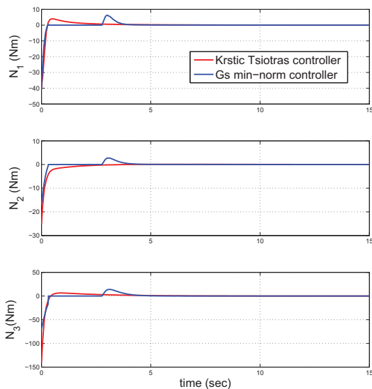
Fig. 4: Control torque comparison between the gain scheduled and the Krstic/Tsotras controllers.
