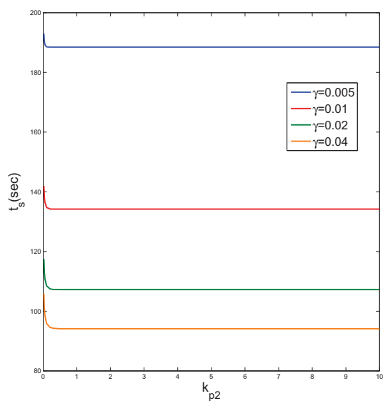
Fig. 9: Settling time as a function of control parameters.
