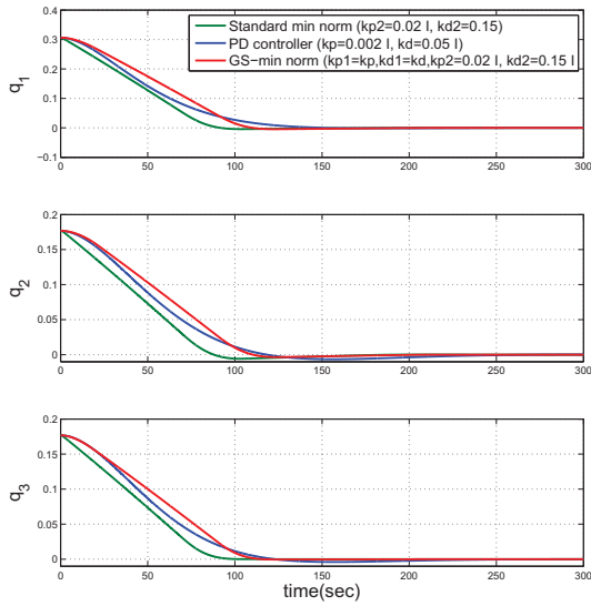
Fig. 2: Attitude response with high gain min norm controller ‘green’, gain scheduled controller ‘red’ and with PD controller ‘blue’.
