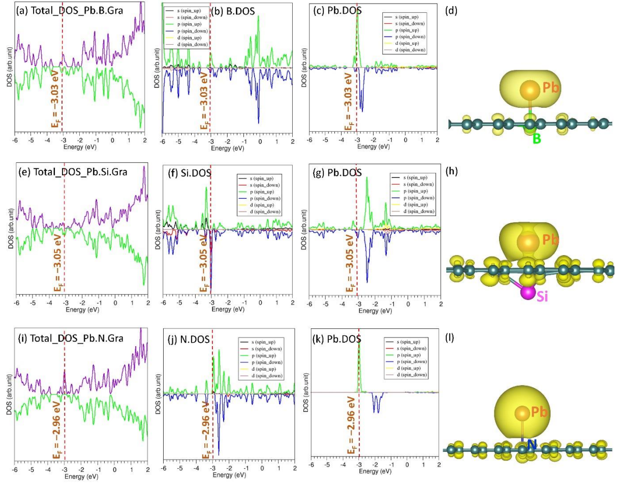
Figure 6. (a) Total DOS plot calculate for the B-doped graphene, (b) atomic DOS plot of B (c) atomic DOS plot of Pb and (d) constant charge density plot associated with the Pb and its neighbour C atoms. Similar plots are shown for Si (e-h) and N (i-l).
