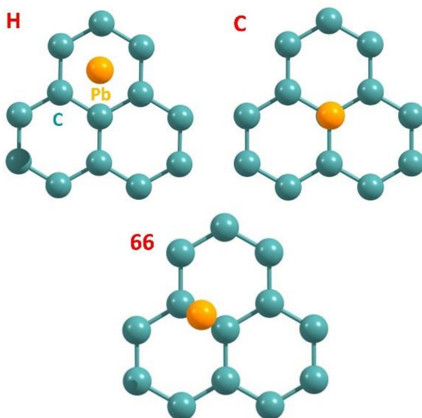
Figure 1. Initial configurations of a single Pb atom adsorbed on the pristine graphene.
