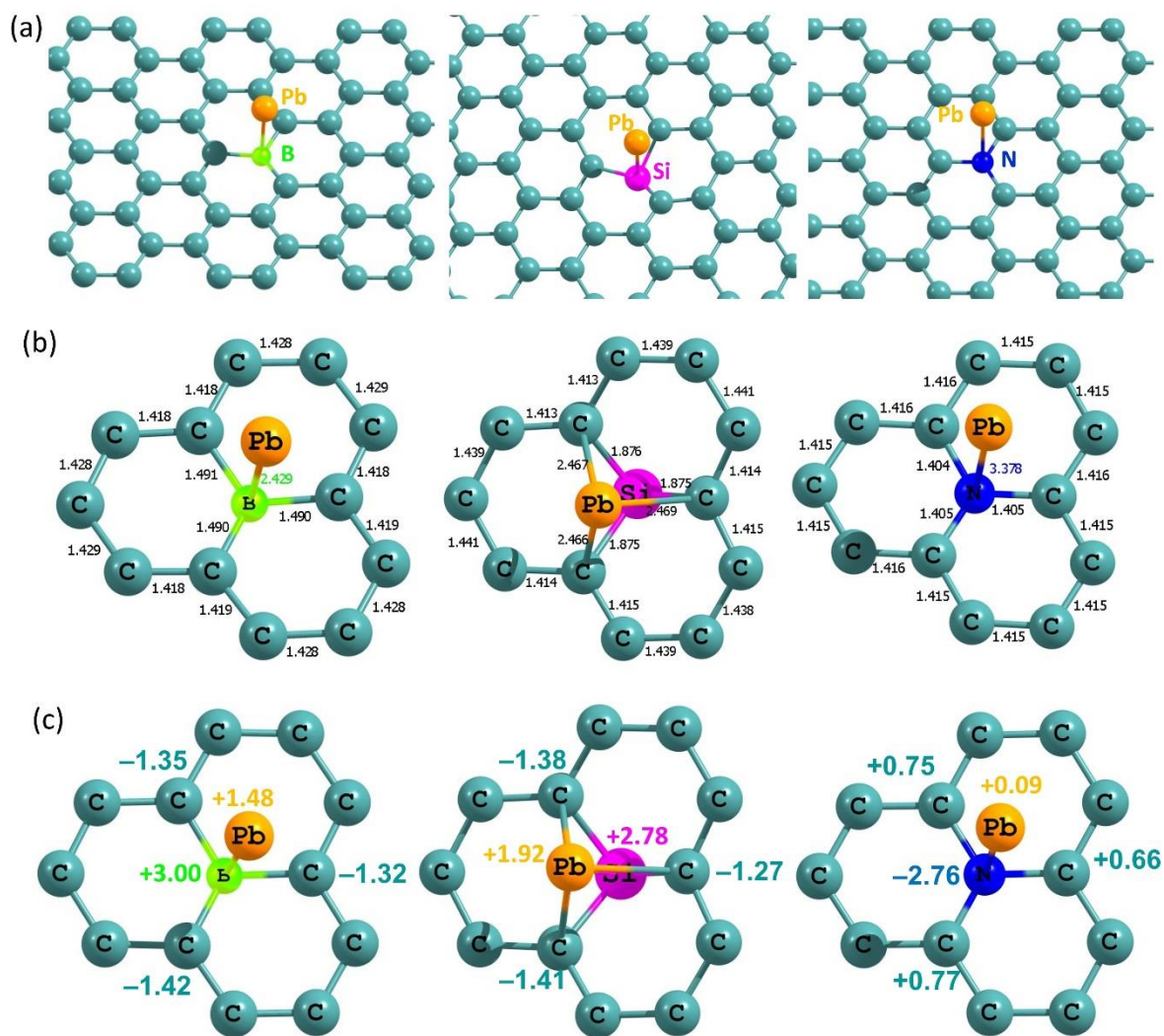
Figure 5. (a) Relaxed configurations of Pb adsorbed on the surfaces of B, Si and N doped graphene, (b) bond distances around the doped atoms and (c) Bader charges on the doped atoms, the Pb and the C atoms attached to them.
