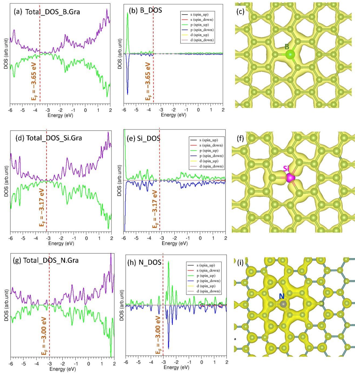
Figure 4. (a) Total DOS plot of B-doped graphene, (b) atomic DOS plot of B and (c) constant charge density plot associated with the B atom and its neighbour C atoms. Similar plots are shown for Si (d-f) and N (g-i).
