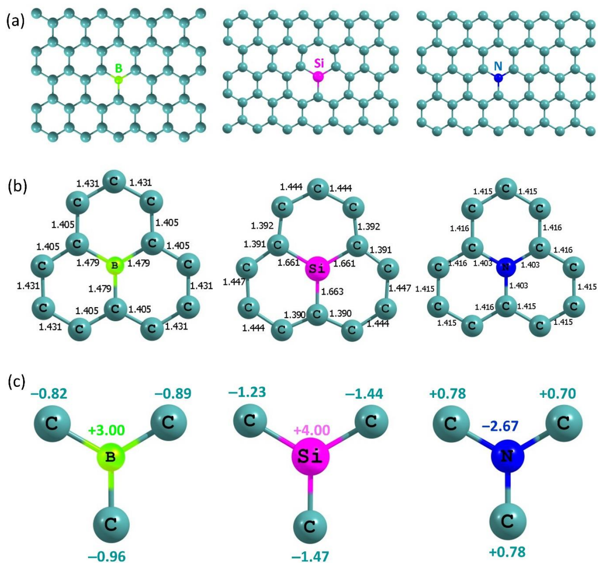
Figure 3. (a) Relaxed configurations of B, Si and N doped graphene, (b) bond distances around the doped atoms and (c) Bader charges on the doped atoms and C atoms attached to them.
