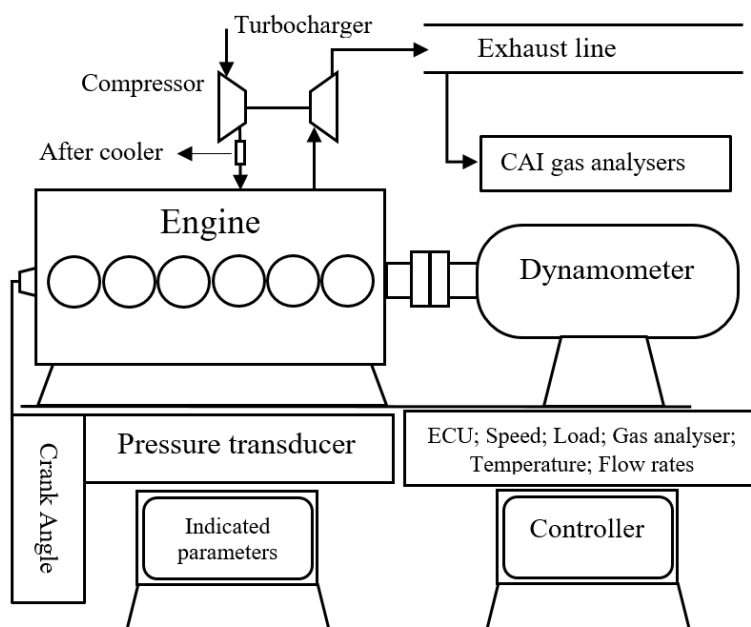
Figure 1 Schematic diagram of test set-up
