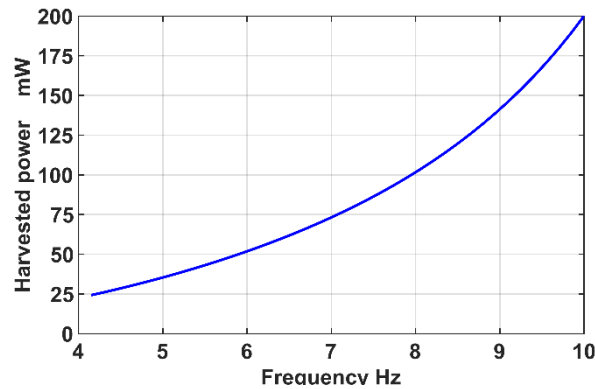
Figure 11. Harvested power frequency responses for all the piezoelectric sensors bonded on the upper surface and lower surface of the wing
