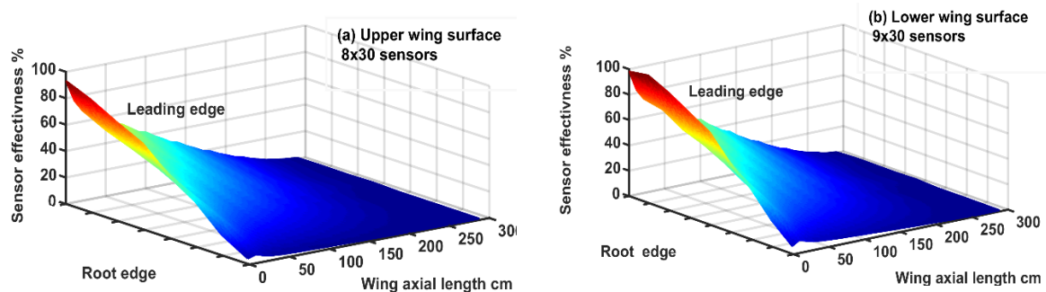
Figure 5. Percentage sensor effectiveness distribution over upper and lower surface of the wing
