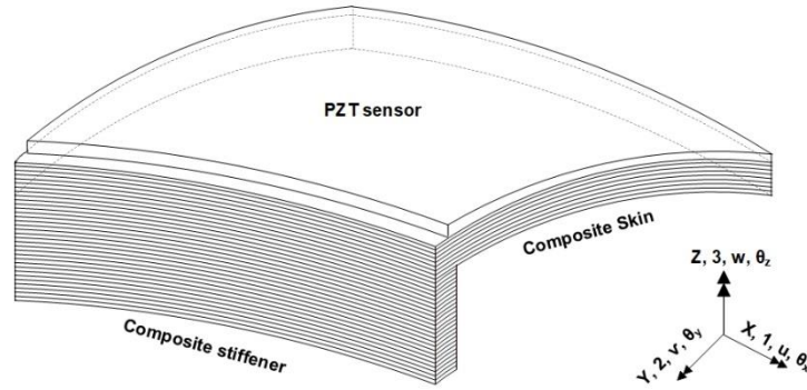
Figure 1. Wing skin element stiffened by beam bonded piezoelectric sensor
