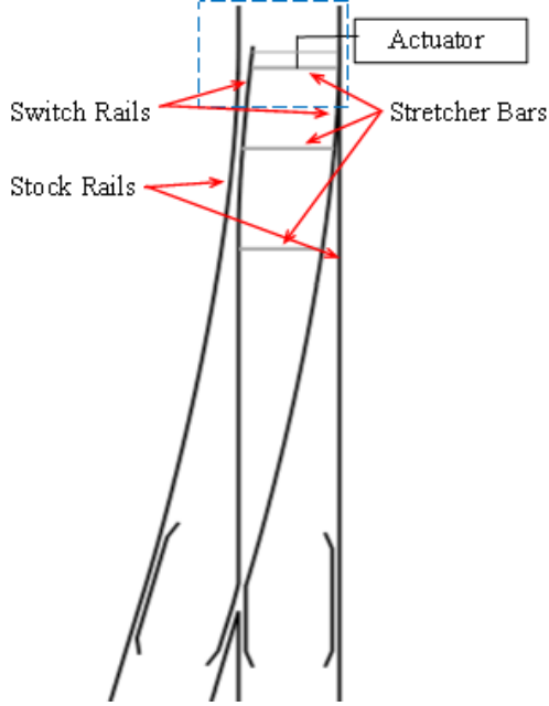
Fig. 1 The switch Layout
