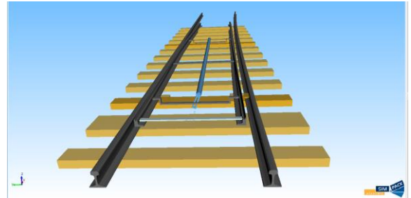
Fig. 3 MBS model of the switch system developed in Simpack
