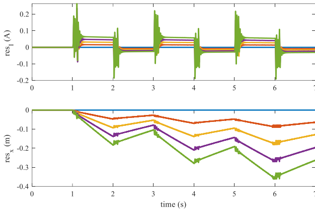
Fig. 5 Input Voltage and Residuals (motor current and displacement) under the different health conditions
