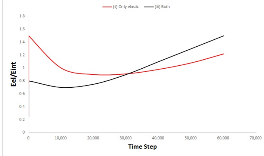
Figure 3: Evolution of ratio of total elastic strain energy to total interfacial energy under different conditions.
