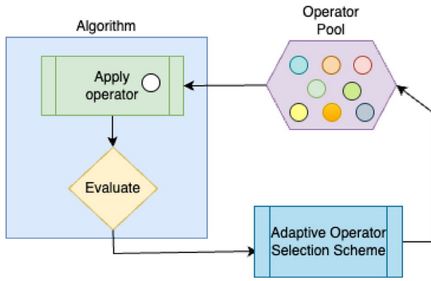
Fig. 3 Adaptive operator selection process trained with supervised machine learning algorithms interacting with ABC algorithm in each bee generation
