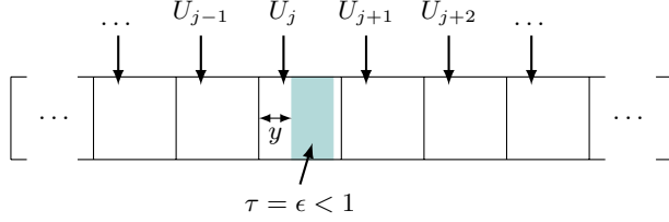
FIG. 18. Visualization of systematic resampling
